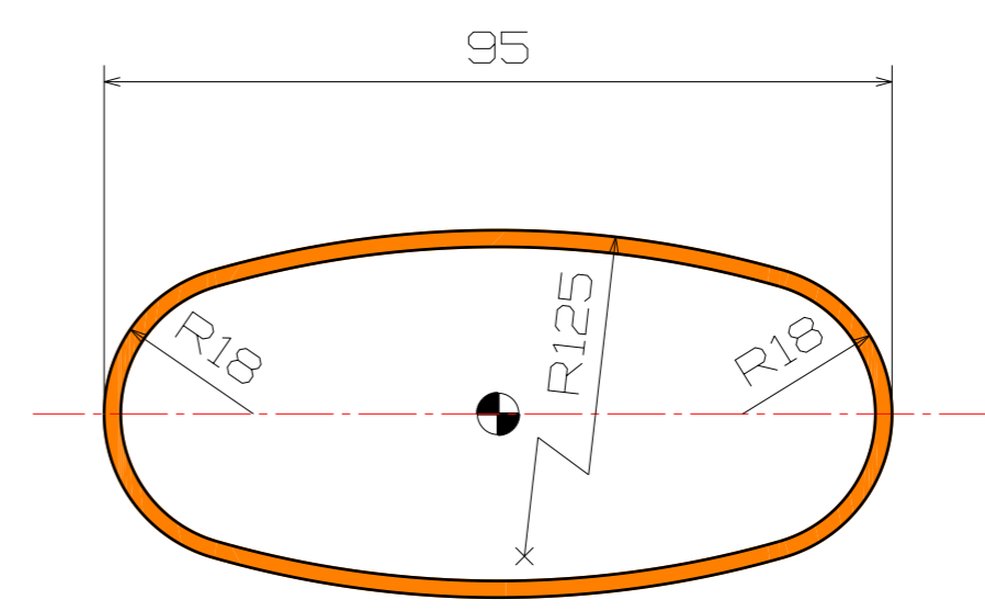
Section cut B-B
