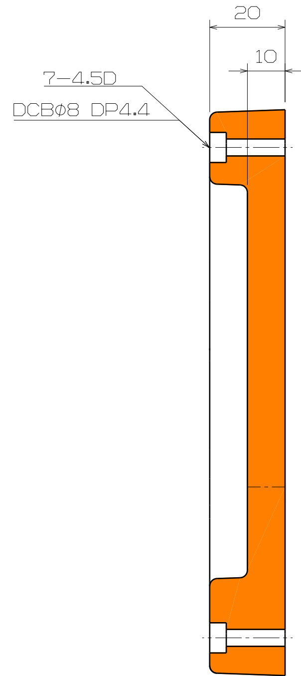
Section view A-A
