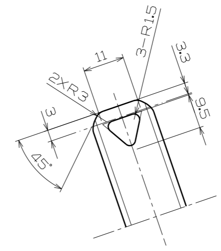
Auxiliary View B
