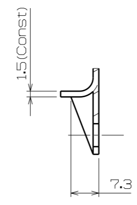
Section View A-A
