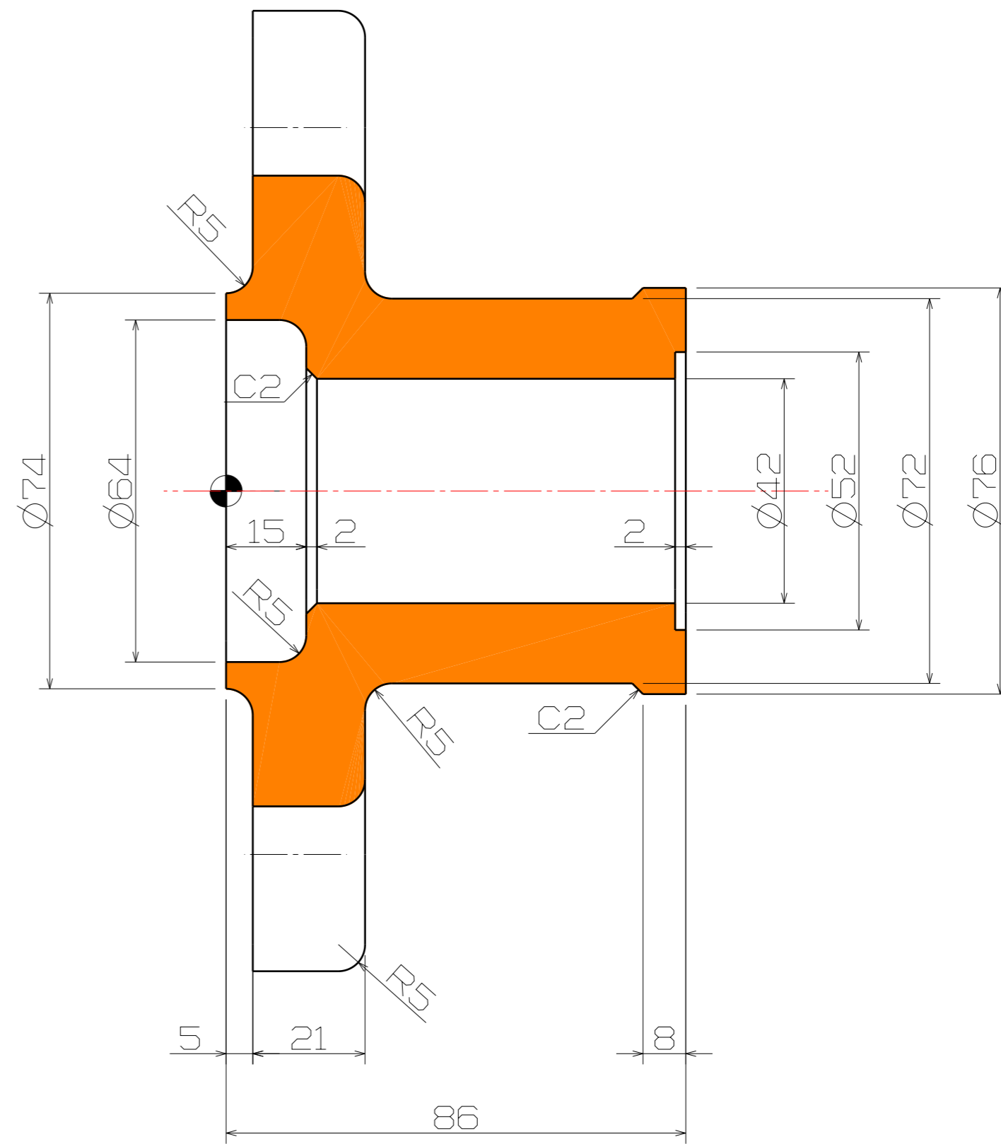
Section view A-A
